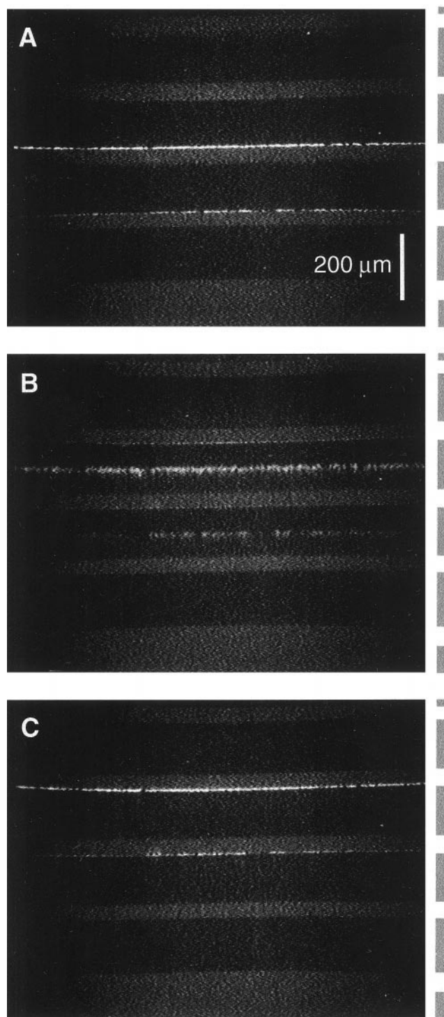
FIGURE 5 Controlled movement of DNA molecules from one trap to another. (A) Applying a purely oscillating field traps molecules over an edge. (B) Mixing a pulse of constant voltage with the oscillating trapping voltage dislodges molecules from the trap, moving them upwards in the image. (C) The pulse duration is chosen so that molecules travel just far enough to settle into the next trap. Gray bars on right indicate the positions of the strips of gold film in the figures. Molecules could also be made to move along the traps by applying the oscillating trapping voltage perpendicular to the gold-film strips while a slight steady voltage was simultaneously applied parallel to the strips (data not shown).
